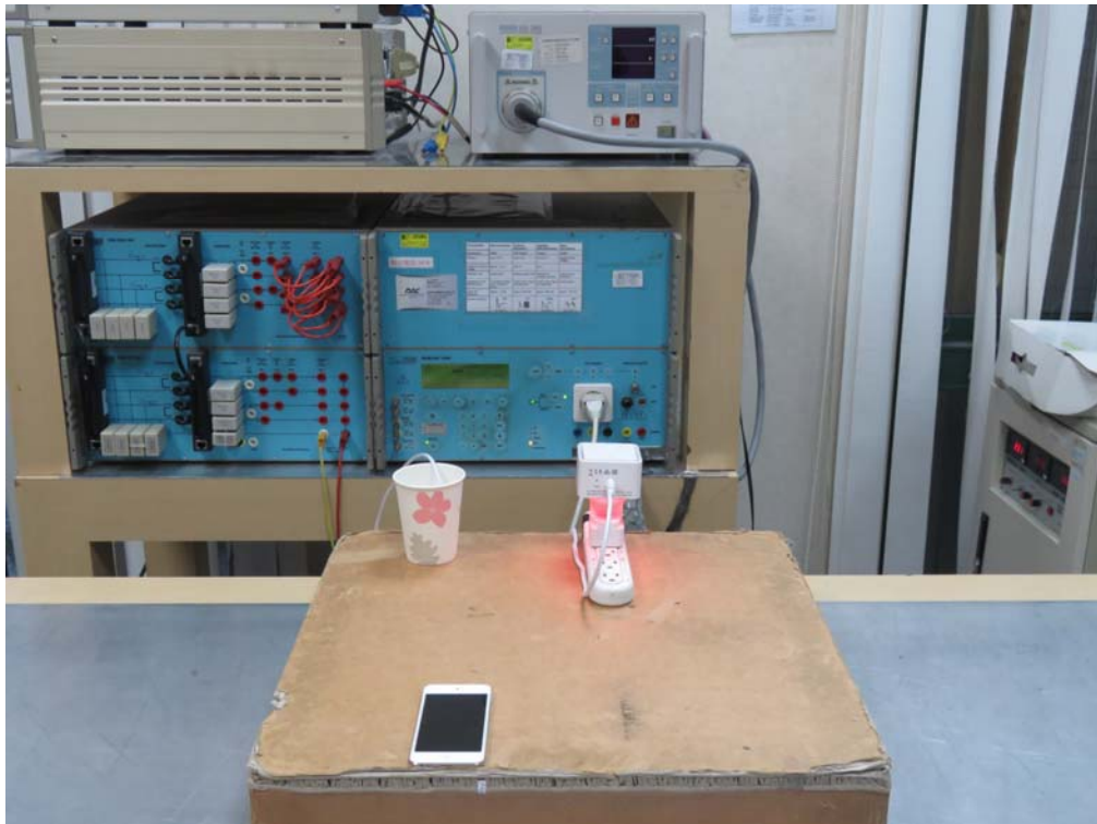
Set Up Photo of EFT & V-DIPS
