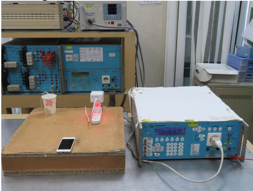
Set Up Photo of Surge
