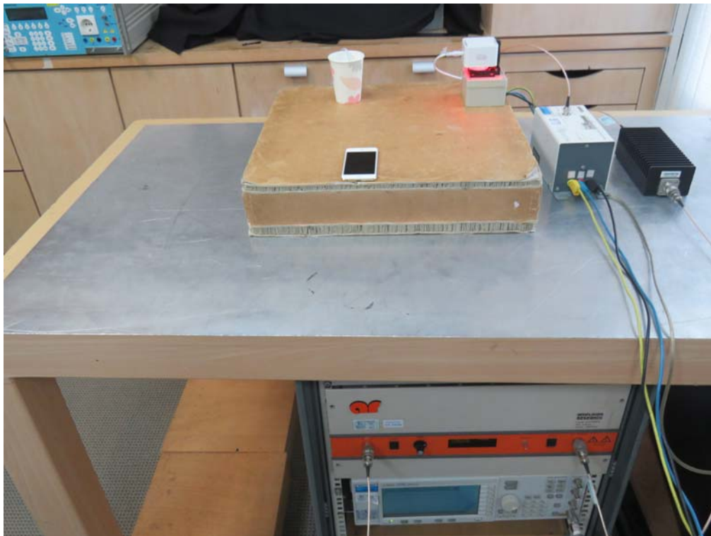
Set Up Photo of CS
